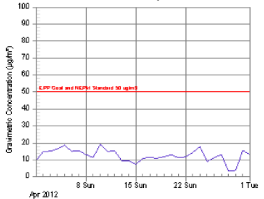
PM 10 Northey St 24 Hour averages
