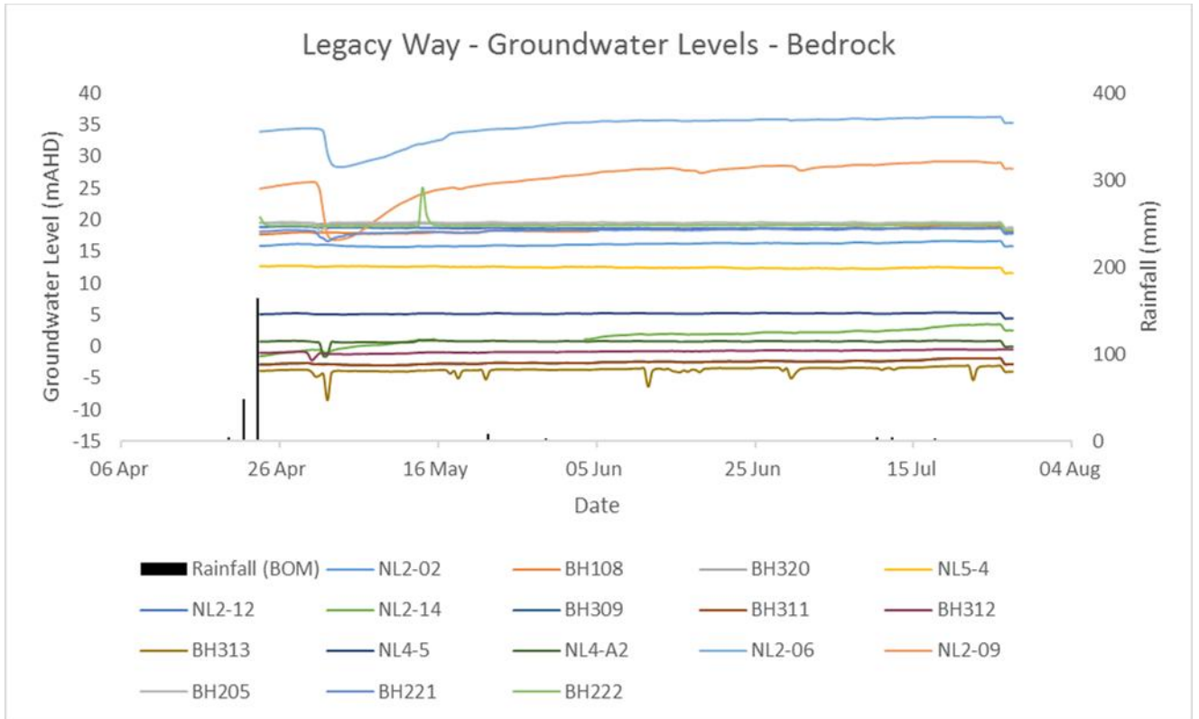
FIGURE 1 - GROUNDWATER LEVELS - BEDROCK
