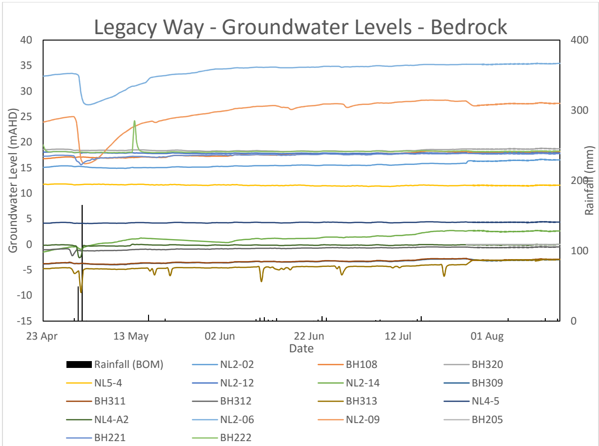
FIGURE 1 - GROUNDWATER LEVELS – BEDROCK
