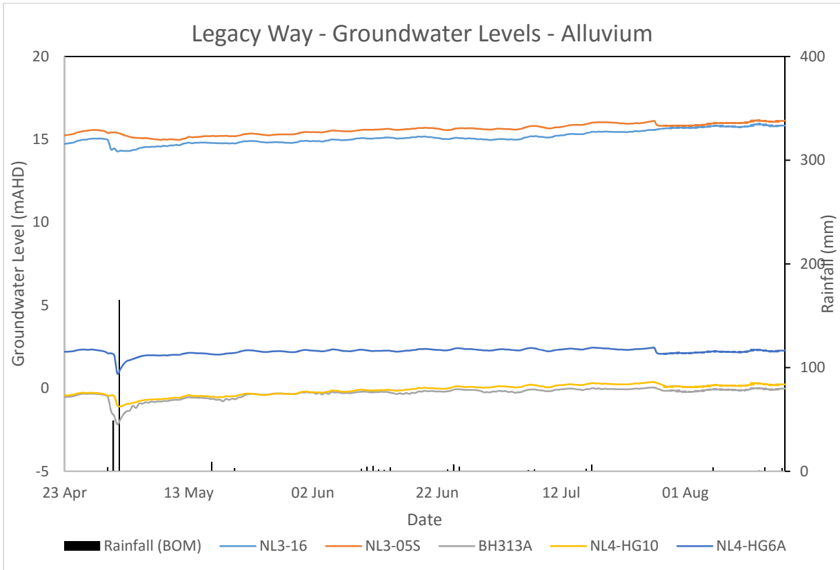
FIGURE 2 - GROUNDWATER LEVELS - ALLUVIUM
